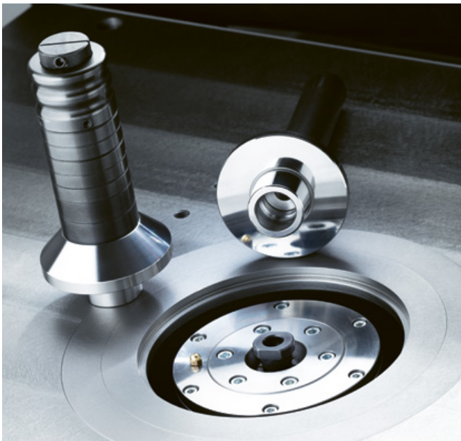
HSK 63 F cutter arbor clamping system | Txx70_63F
