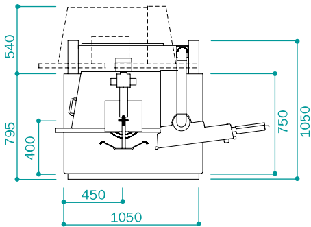
T12 | Plan view
